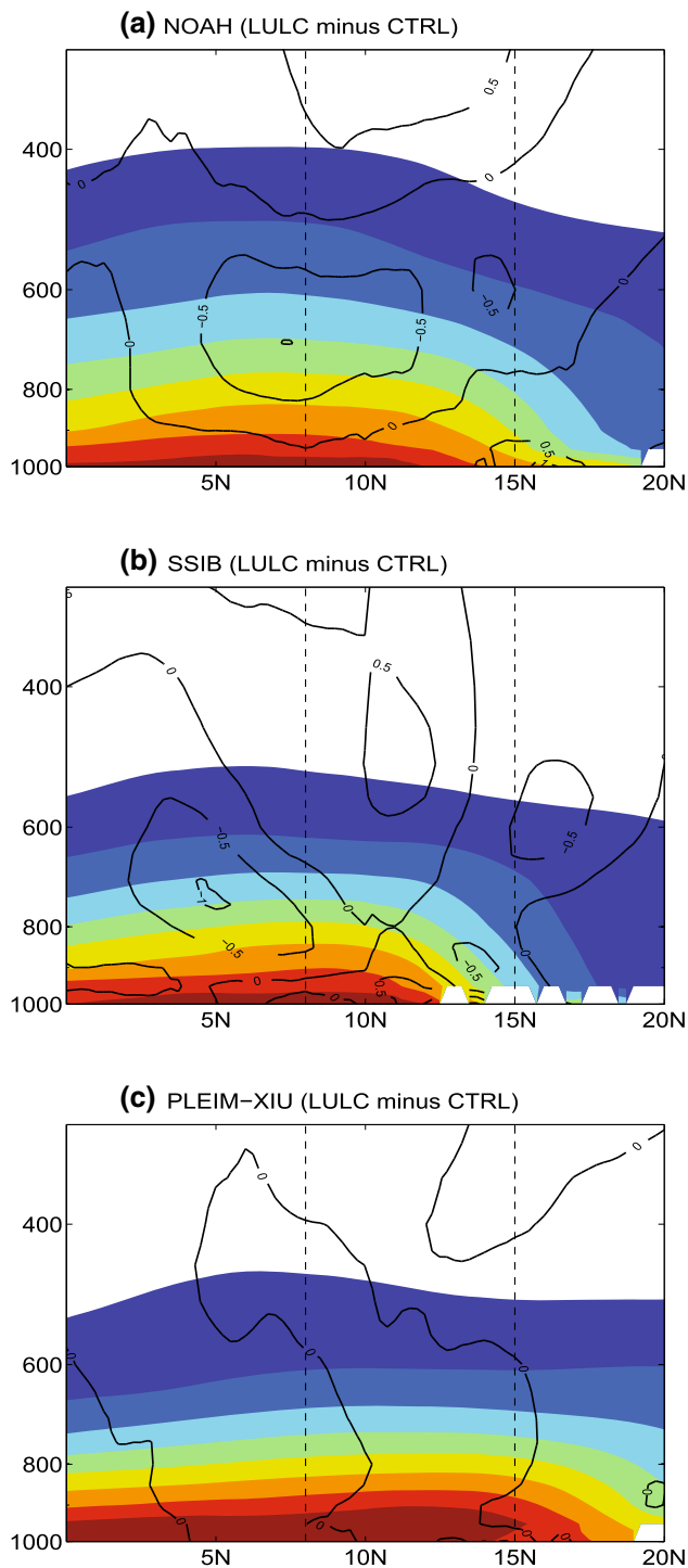
Fig. 10 The change in JJAS mean zonal wind due to the LULC change (contours, m/s) and the LULC water vapor mixing ratio (shaded, g/kg)
