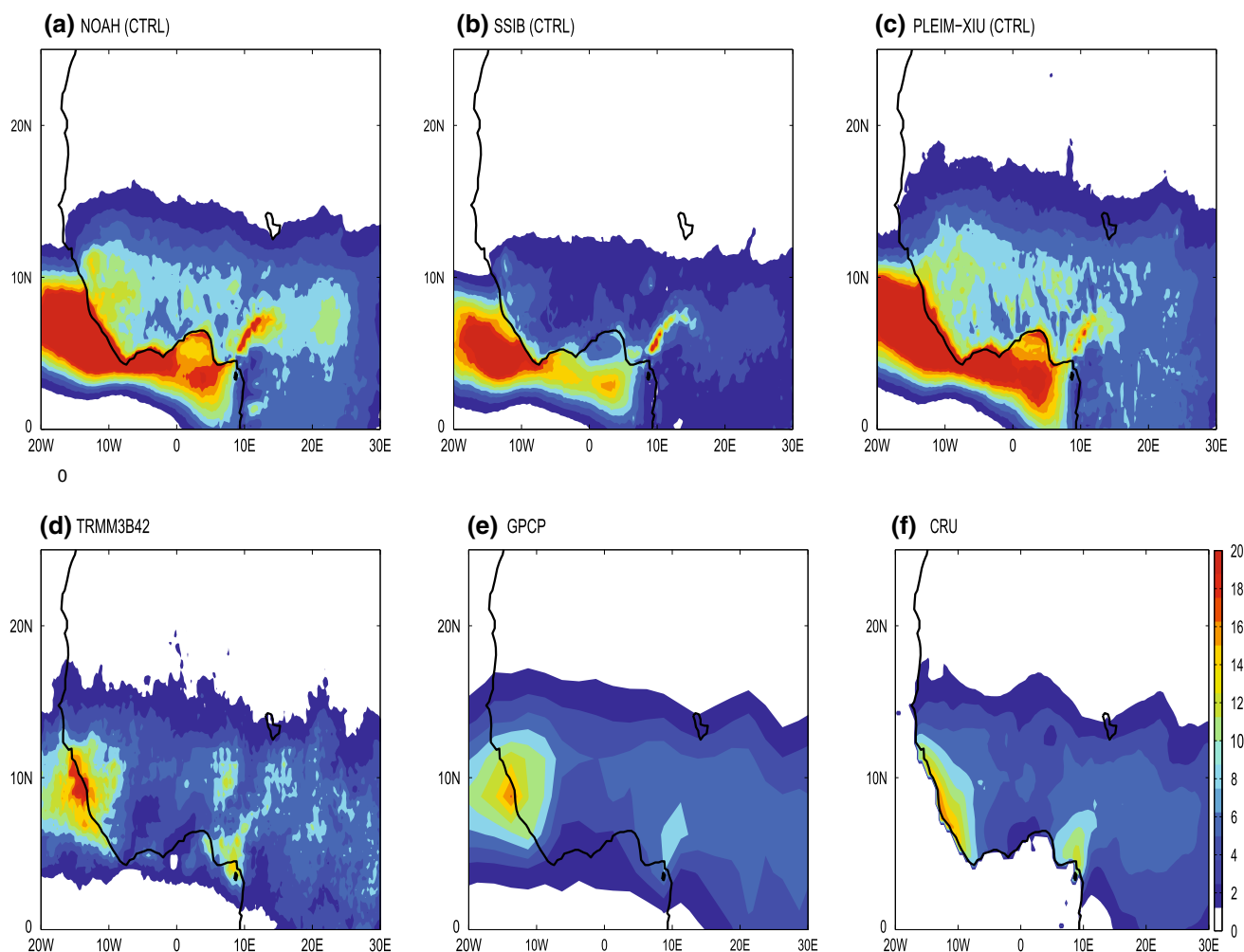
Fig. 3 Comparison of the ensemble means of the JJAS average precipitation (mm/day) from the CTRL simulations with observations
